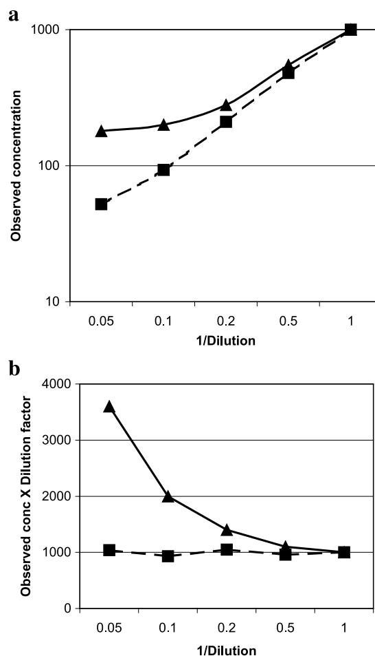
Fig. 6. Parallelism. Data from two individual samples to show parallelism (■) or the lack of it (▲). The same dataset was plotted as (a) observed concentration vs. 1/dilution factor, or (b) dilution adjusted concentrations vs. 1/dilution factor.
