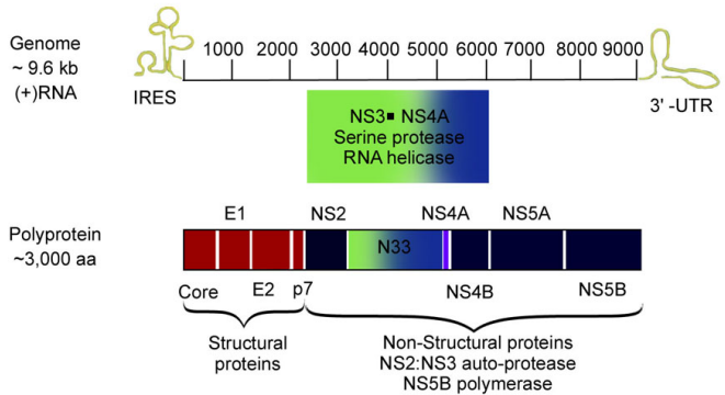
HCV Genome and Polyprotein Potential Drug Targets
